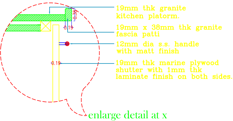
sectional plan of kitchen
