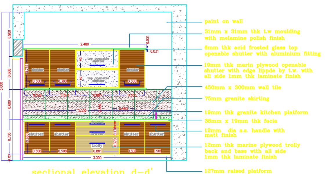
sectional elevation d-d'
