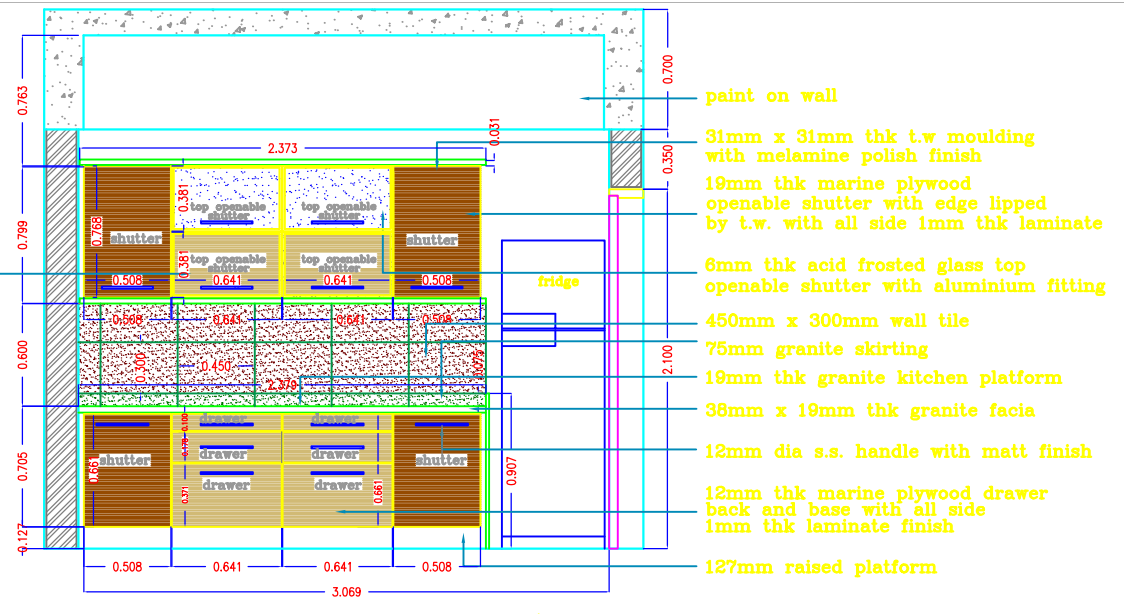
sectional elevation b-b'
