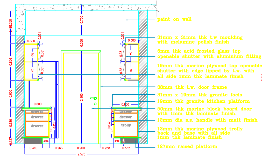
sectional elevation c-c'
