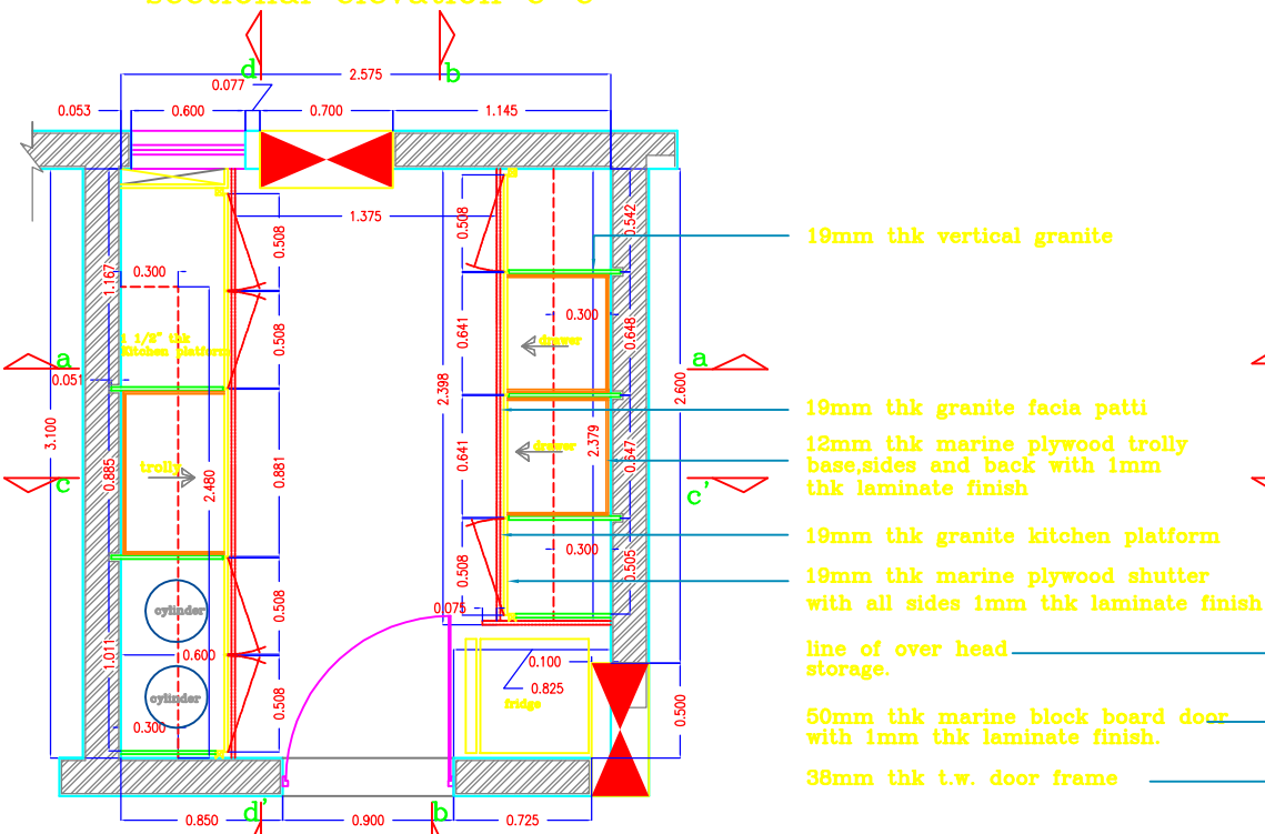
sectional plan of kitchen
